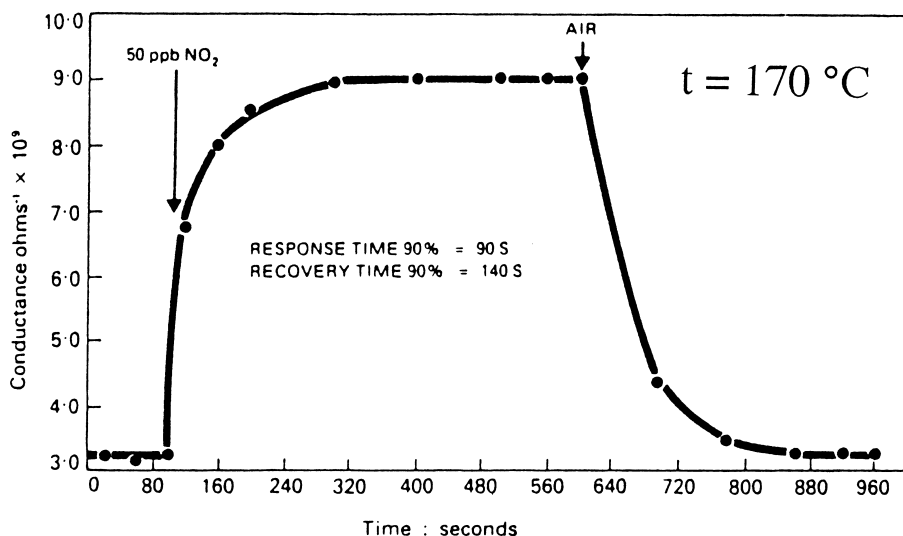
Fig. 15. Variation of the conductance of a PcPb film at 170^\circ\text{C} ( e=8000\text{ \AA} ) under 50 ppb of \text{NO}_2 and return to air (after Ref. [48]).
