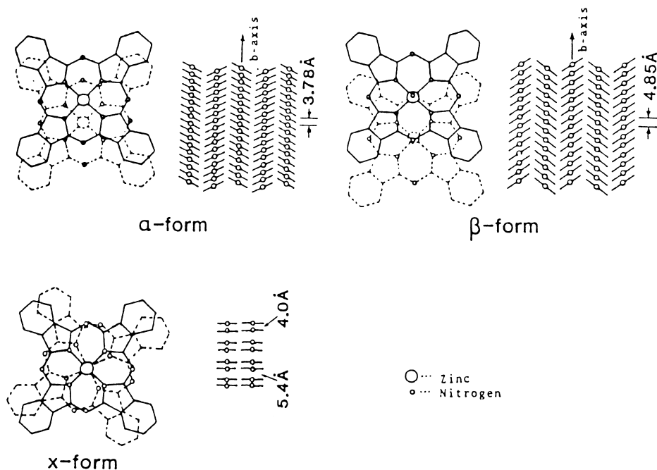
Fig. 2. Schematic representation of the three main molecular stackings found for \text{PcZn} , which is representative of metallophthalocyanines (after Refs. [15–17]).
