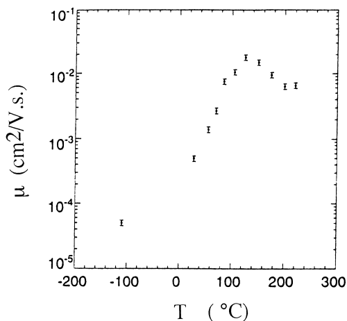
Fig. 42. Field-effect mobility of PcCu at different substrate temperatures. Device n-Si/SiO 2 /PcCu (channel lengths 12 and 25 \mu m) [125]. Rate of deposition = 4 – 5 Å s −1 , pressure = 2.0 \times 10^{-6} Torr.
